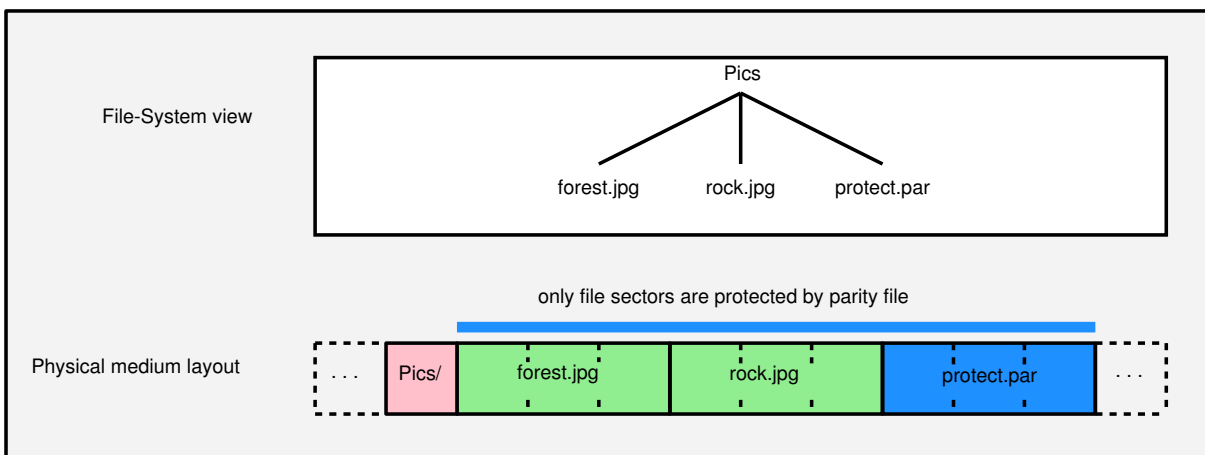
Figure 65: Relation between file system and sectors on the medium.
